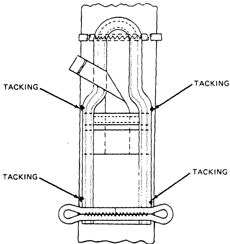
Figure 2-60. Parachute Inspection Data Pocket Tacking Details.
