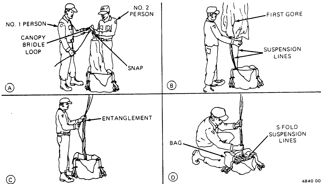
Figure 2-7. Shakeout
