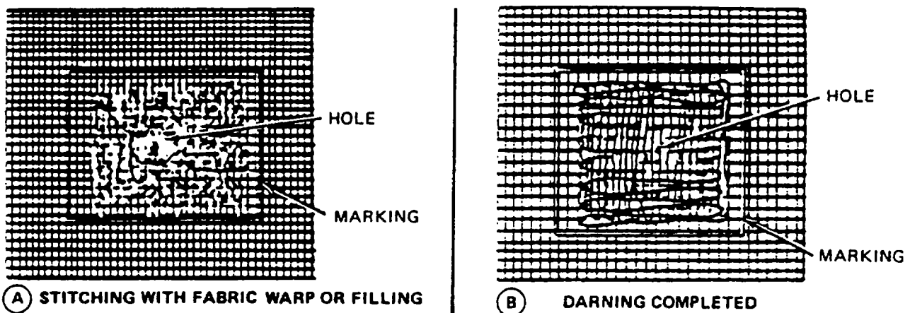
Figure 2-39. Darning Method Using a Darning Sewing Machine.
