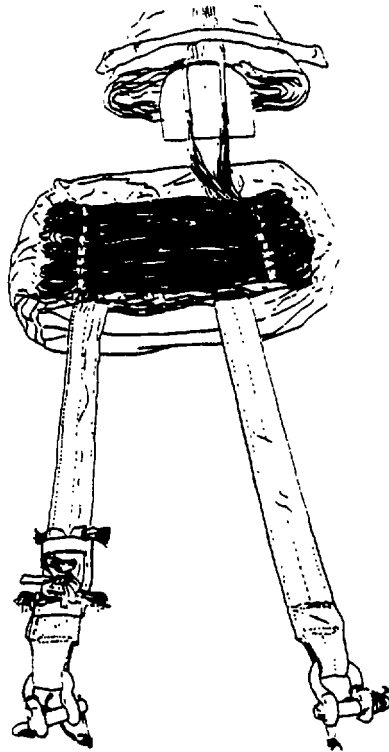
Figure 2-26. Suspension Line Stowage Complete.
